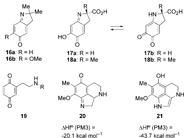
Figure 3. Stable quinoneimines and model compounds.
