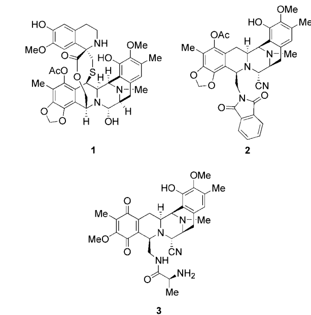
Figure 1. Ecteinasclidin 743 ( 1 ), phthalasclidin ( 2 ), and cyanosafraclin B ( 3 ).
