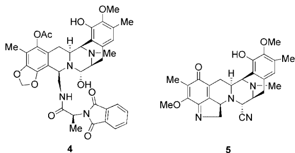
Figure 2. Phthalimido derivative 4 and quinoneimine 5 .
